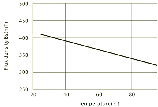
Flux density vs. Temperature
