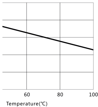
Initial permeability vs. Temperature
