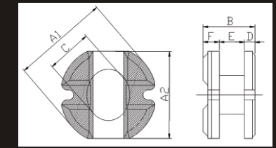
FIG(3) DRR-AxB-EL
